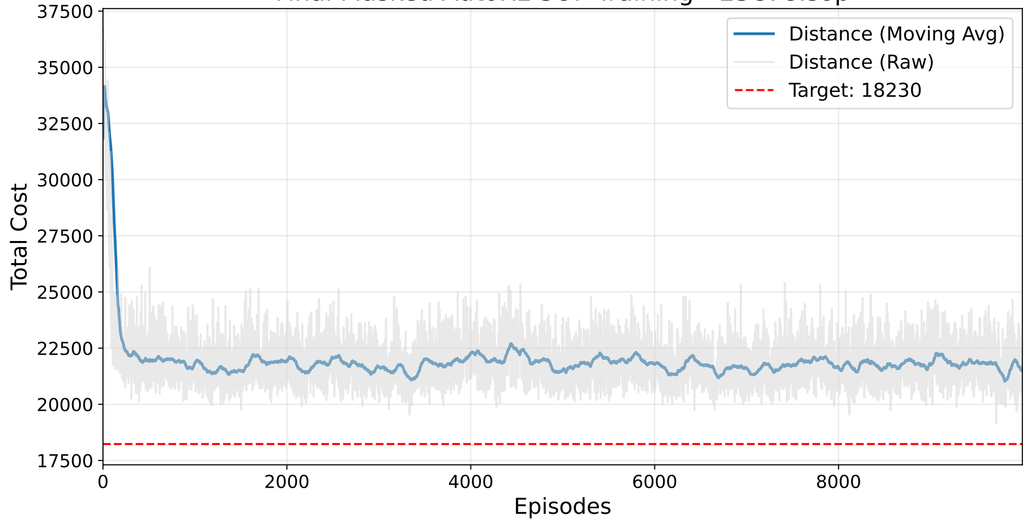
Final Masked AutoRL-SOP Training - ESC78.sop
